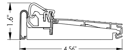
22 INSWING ARTICULATING THRESHOLD ZAC4565RDS
