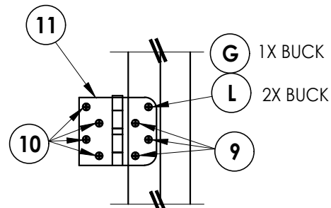
HINGE DETAIL 2
