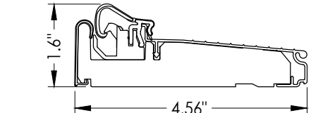
19 INSWING ARTICULATING THRESHOLD ZAC4565FN
