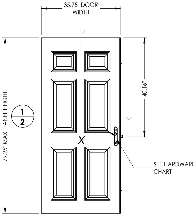
40 DOOR PANEL Plastpro Fiberglass
