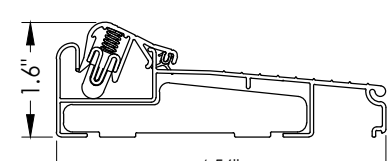
20 INSWING ARTICULATING THRESHOLD ZACLAA4565
