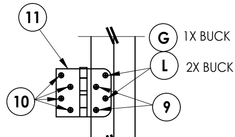
HINGE DETAIL 1
