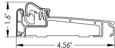
18 INSWING ARTICULATING THRESHOLD ZACL4565
