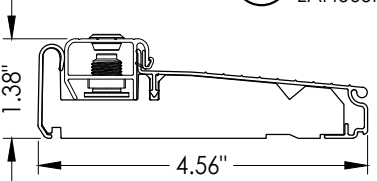
16 INSWING ADJUSTABLE THRESHOLD ZAI4565FN
