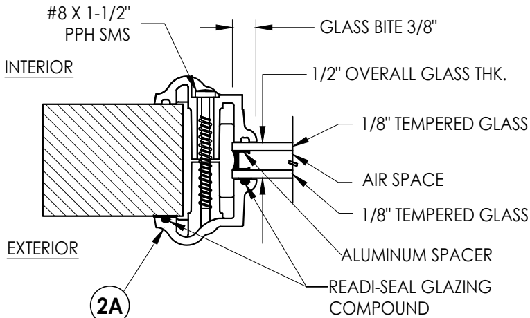
2A G1 GLAZING DETAIL
