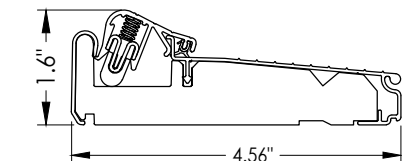
21 INSWING ARTICULATING THRESHOLD ZACAA4565FN
