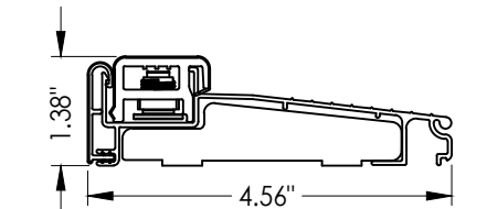
13 INSWING ADJUSTABLE THRESHOLD ZAIL4565
