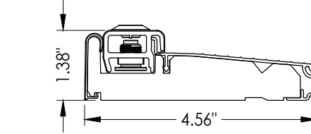
14 INSWING ADJUSTABLE THRESHOLD ZAI4565FN
