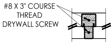
DETAIL 1
