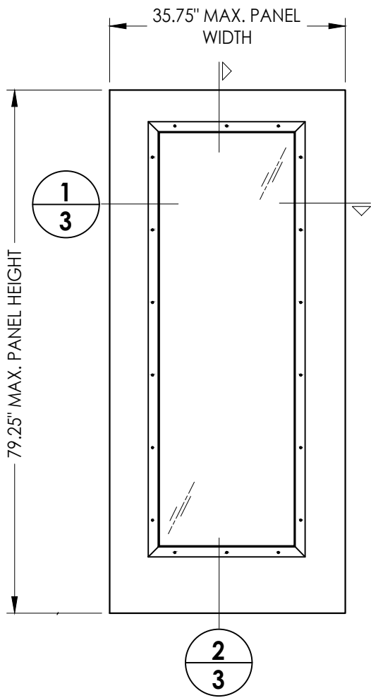
50 SIDELITE PANEL Plastpro Fiberglass
